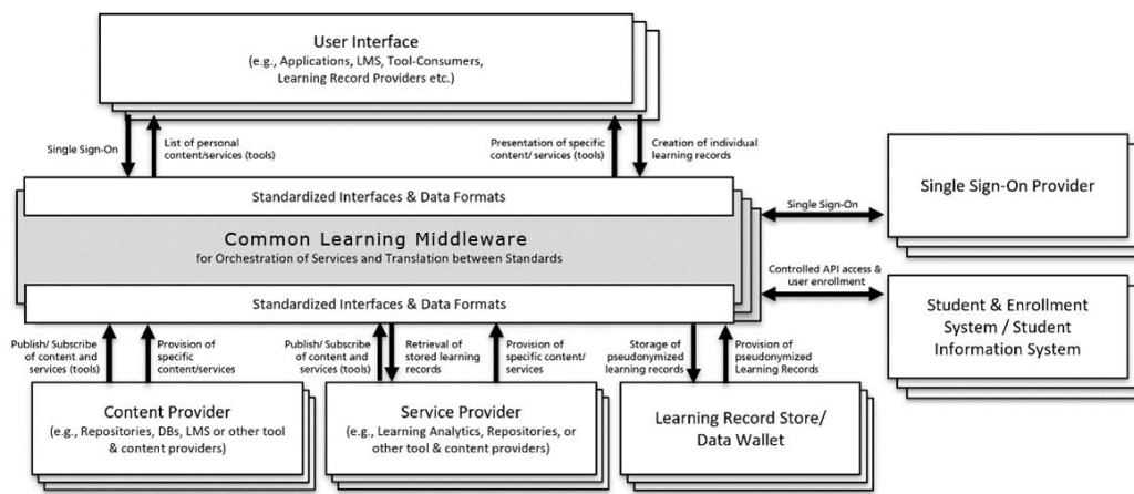
Figure 1: Architecture of the AI-enabling Interoperable Infrastructure
